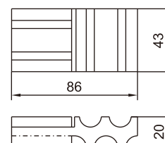
SD1 型隔振垫 0.5 基本块安装尺寸 Dimensions of 0.5 SD1 basic vibration isolated pad
